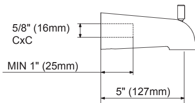
Bath spout / Bec de bain
